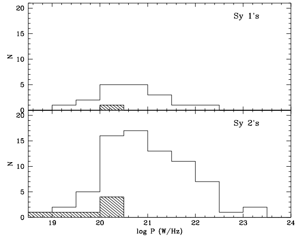
Fig. 19. Histograms of the radio power distribution for Seyfert 1's and Seyfert 2's. Shaded regions represent upper limits.
